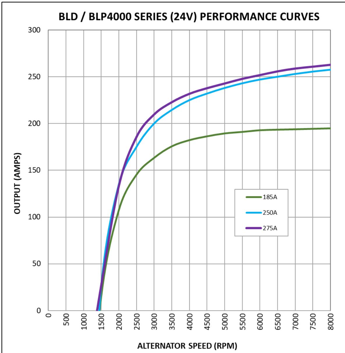
Stabilized output @ 24°C, as per S.A.E. J56
